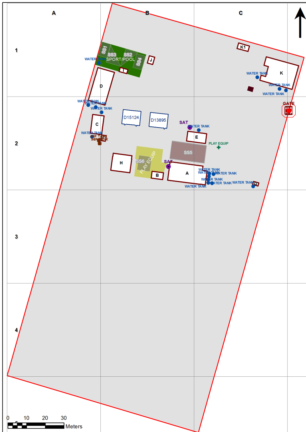
3211 - Tibooburra Outback Public School Site Plan (12876)
