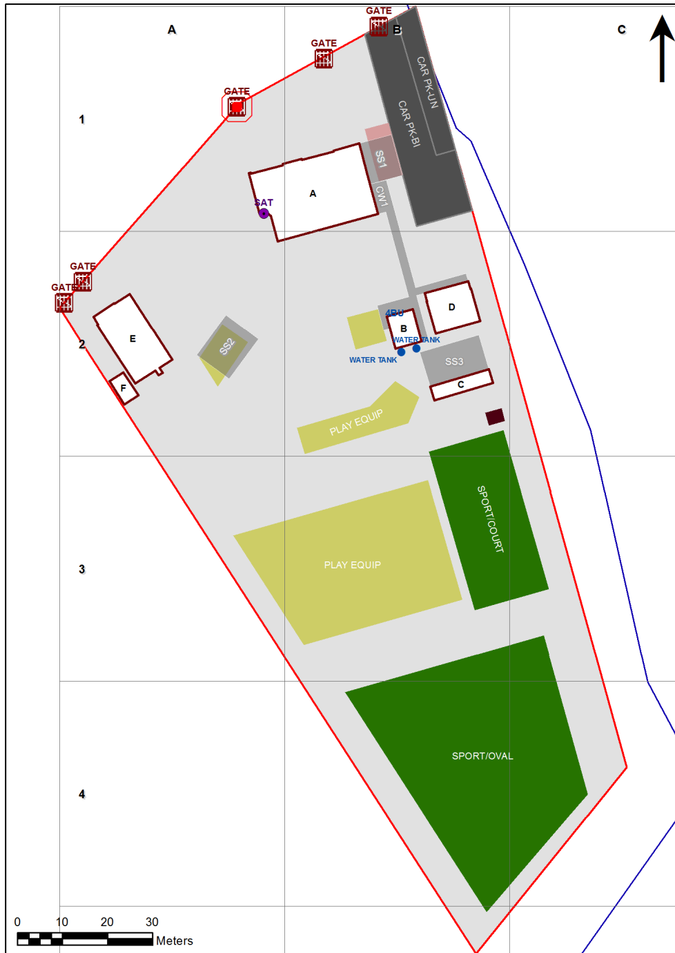
3566 - Zig Zag Public School Site Plan (11423)
