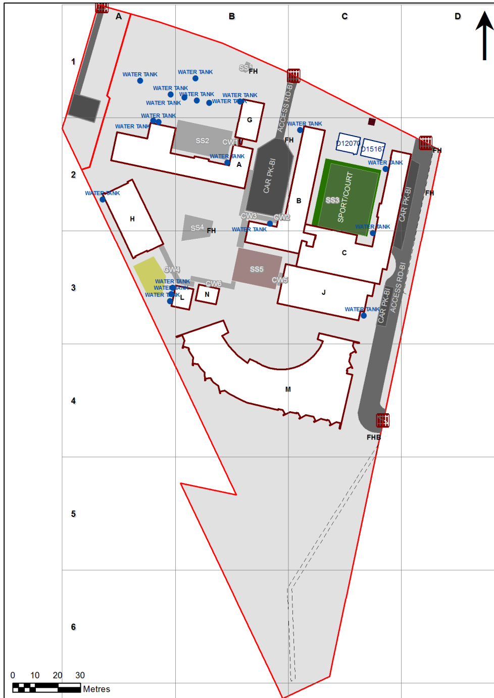
3869 - Yagoona Public School Site Plan (10852)
