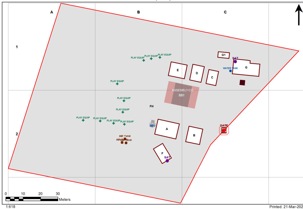
3521 - Wyangala Dam Public School Site Plan (11413)
