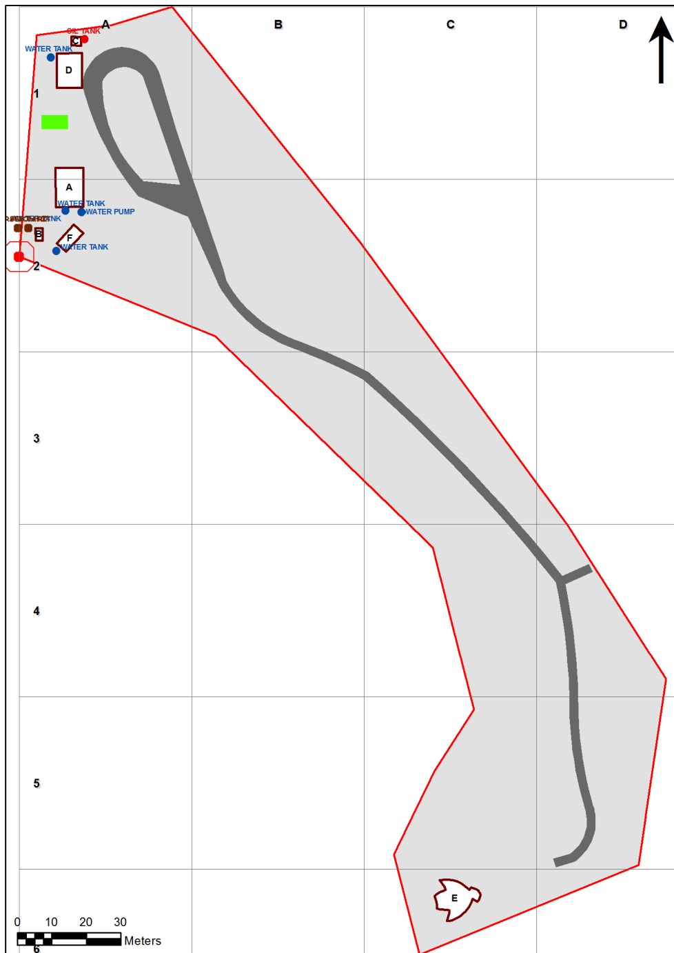
5667 - Wooglemai Environmental Education Centre Site Plan (14567)
