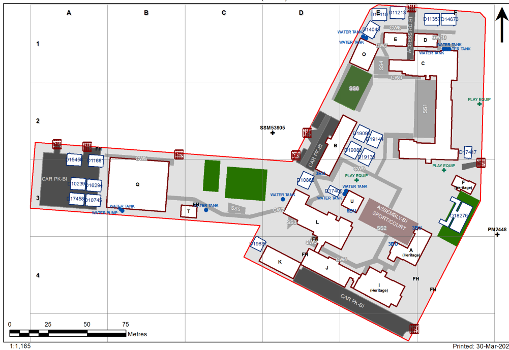
3883 - Westmead Public School Site Plan (12901)
