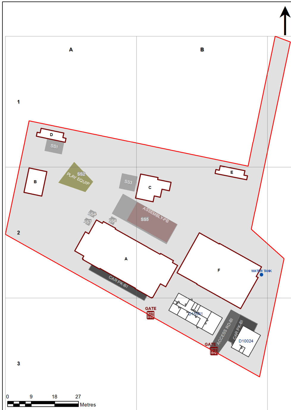
3310 - Undercliffe Public School Site Plan (13123)
