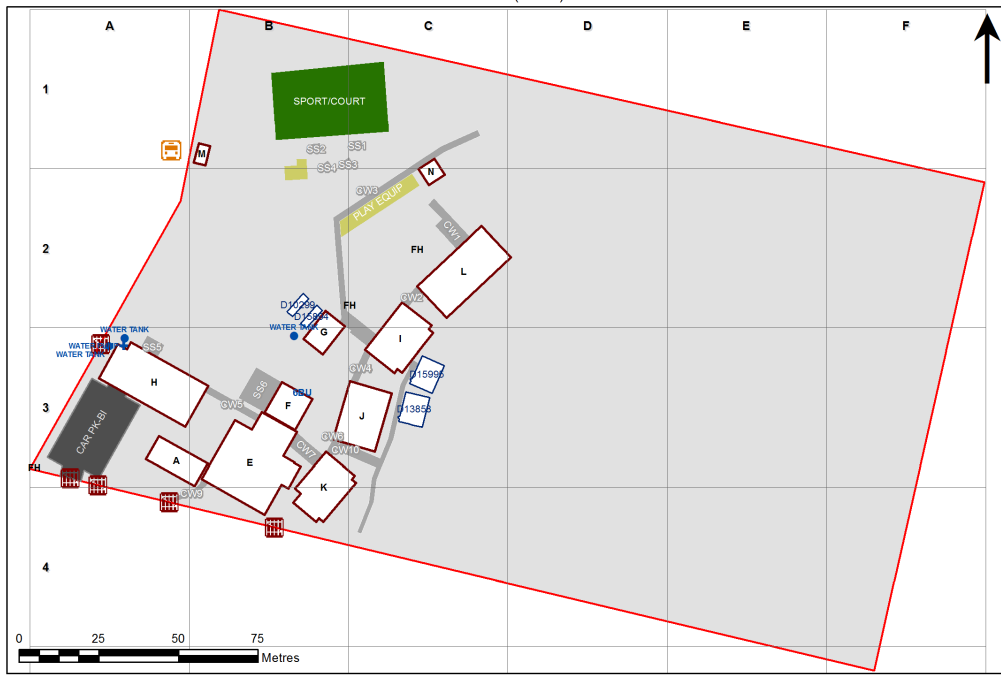
3269 - Tuggerah Public School Site Plan (11499)
