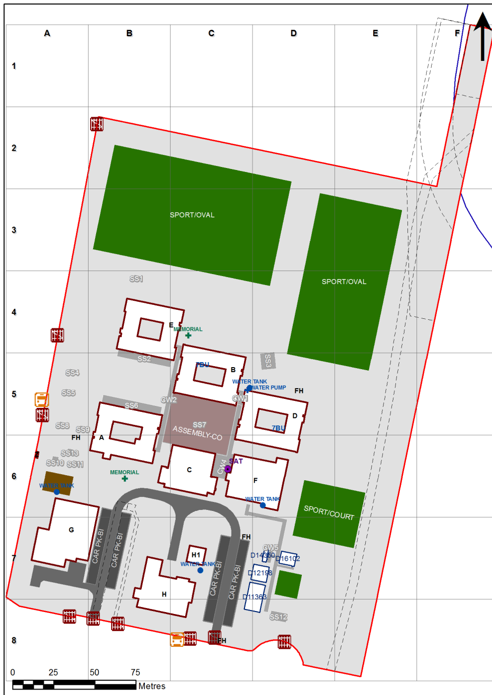
8465 - Tuggerah Lakes Secondary College The Entrance Site Plan (11487)
