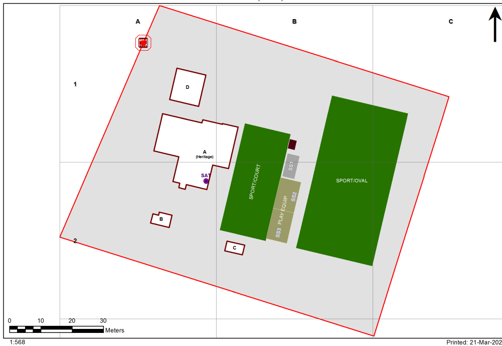
3222 - Tirranna Public School Site Plan (13337)
