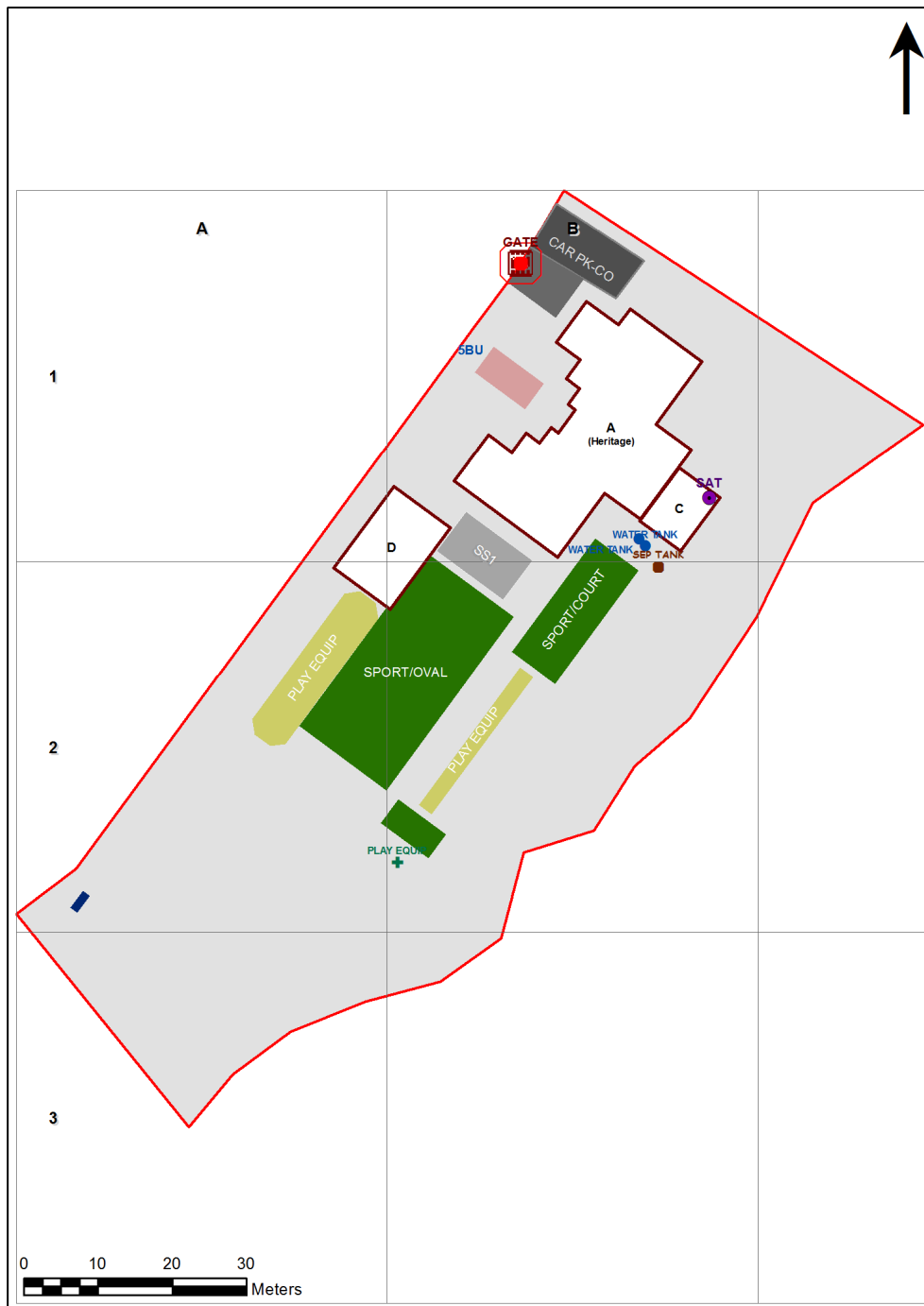
3045 - Scarborough Public School Site Plan (11280)
