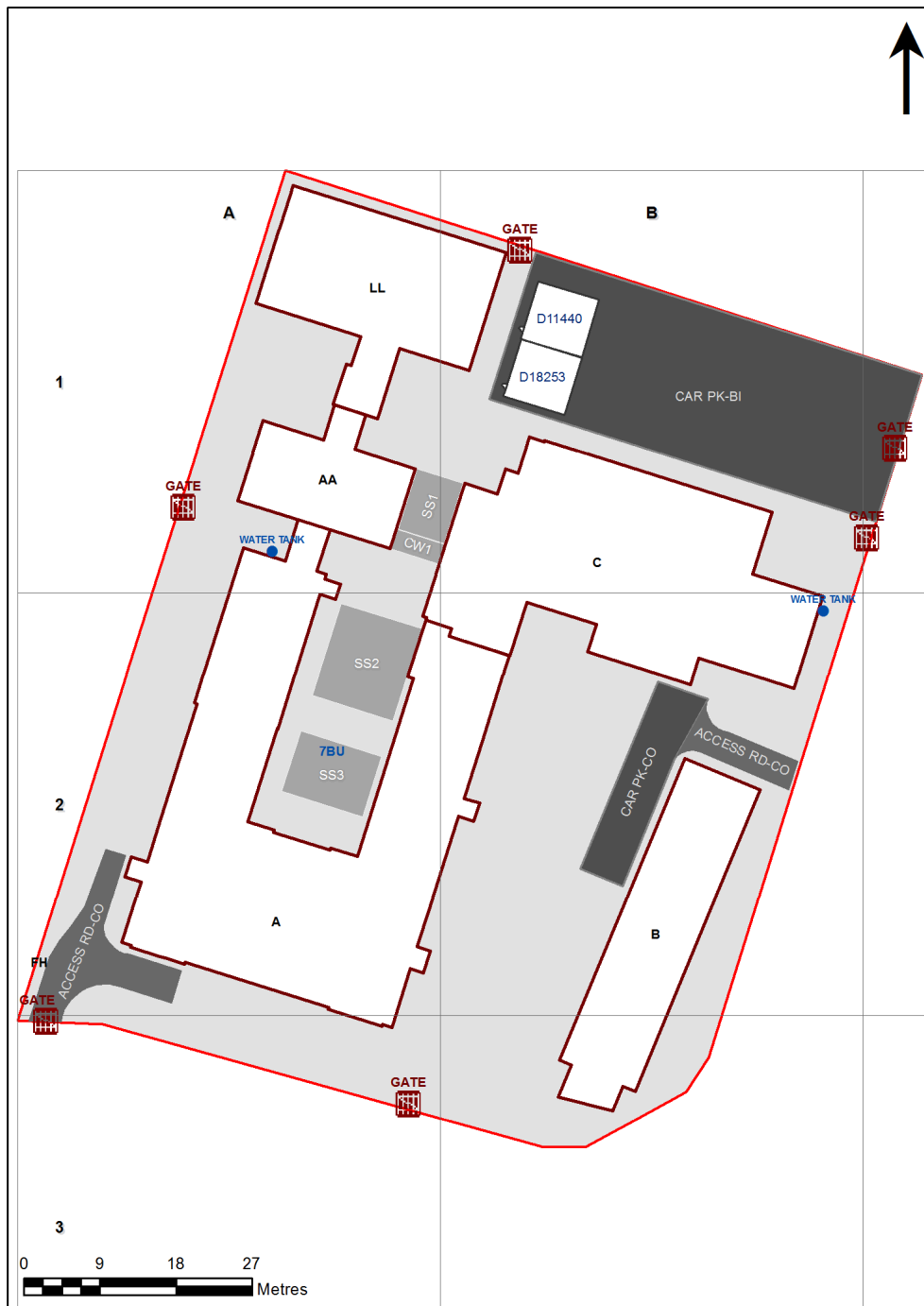
8135 - Parramatta High School Site Plan (12035)
