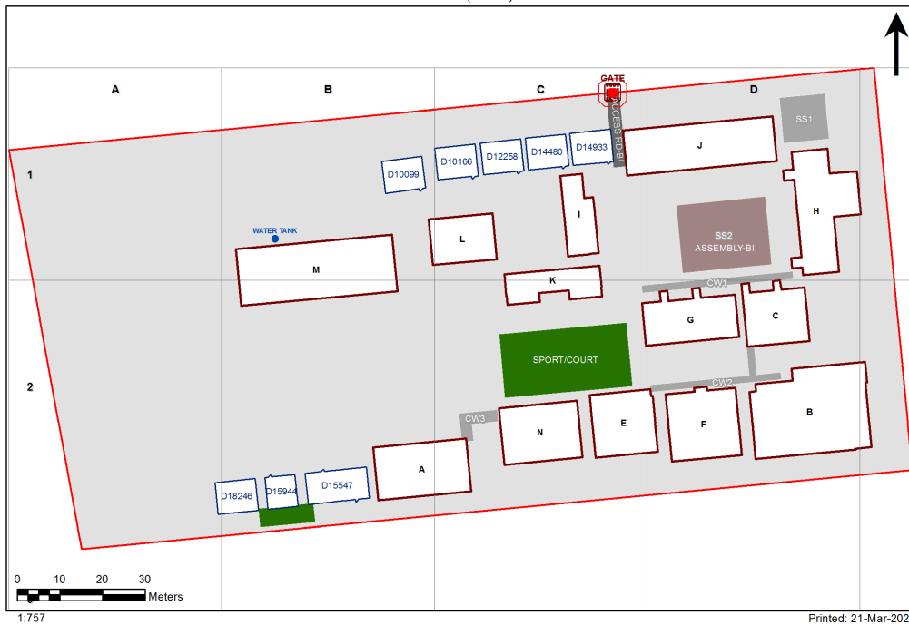
3797 - Oatley West Public School Site Plan (12980)
