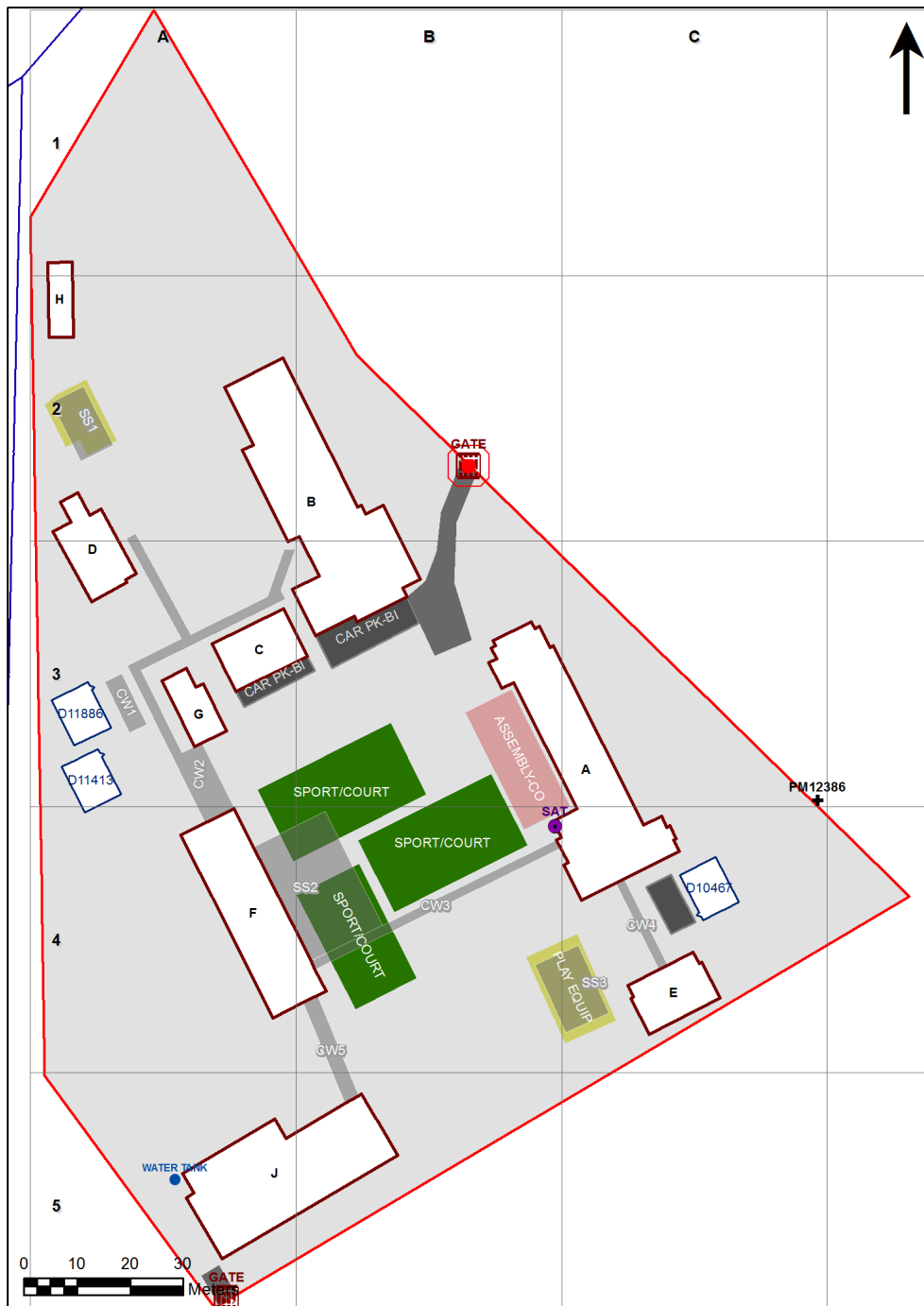
3798 - New Lambton South Public School Site Plan (11561)
