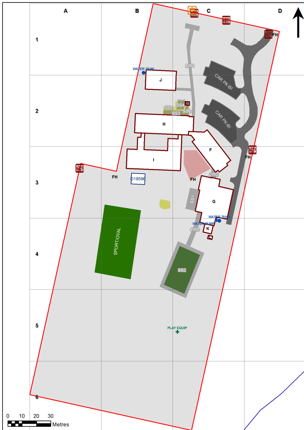
2703 - Narara Public School Site Plan (10499)
