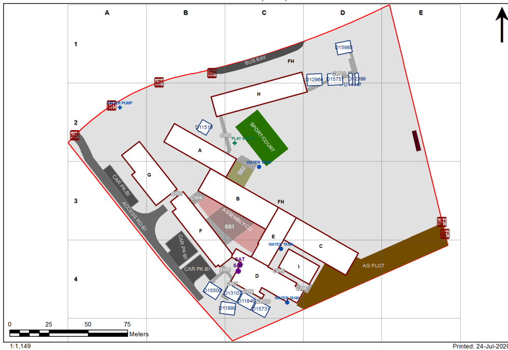
4610 - Mount Terry Public School Site Plan (13604)
