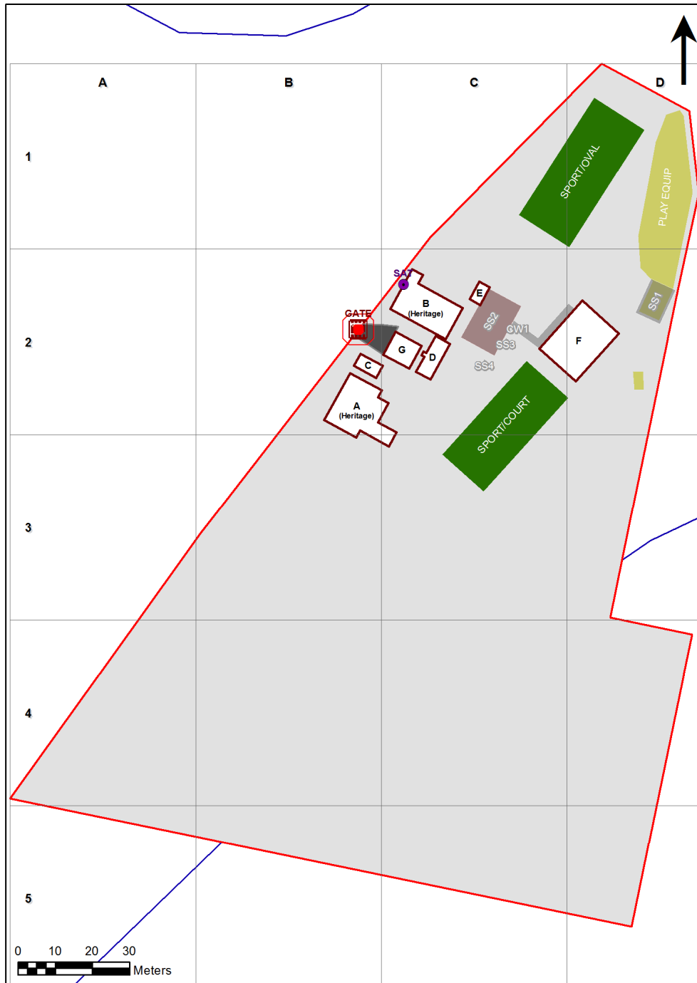
2586 - Mogo Public School Site Plan (11444)
