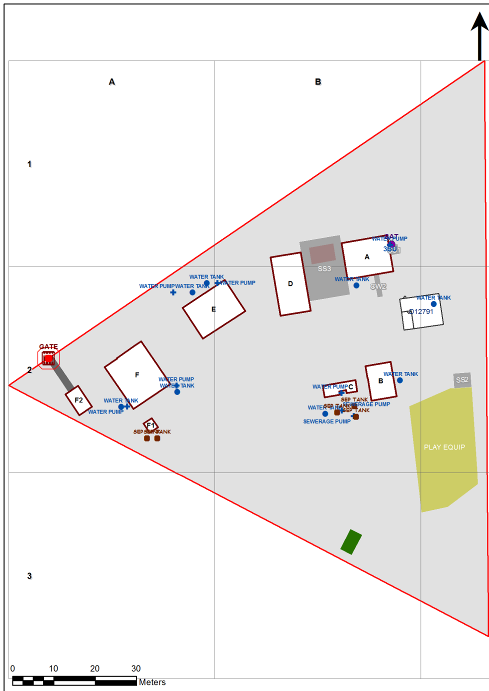
2492 - Martindale Public School Site Plan (12802)
