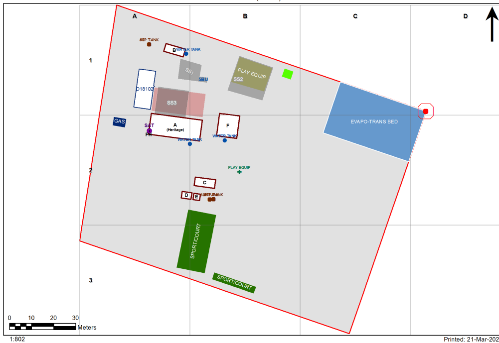
2485 - Marrar Public School Site Plan (11441)
