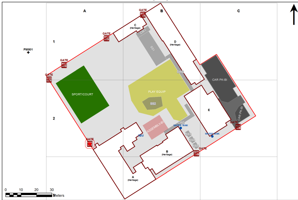
3950 - Manly Village Public School Site Plan (11835)
