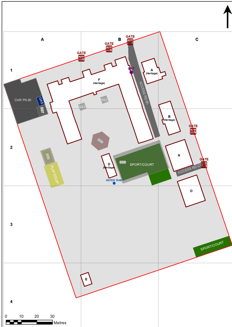
7305 - Manilla Central School Site Plan (12794)
