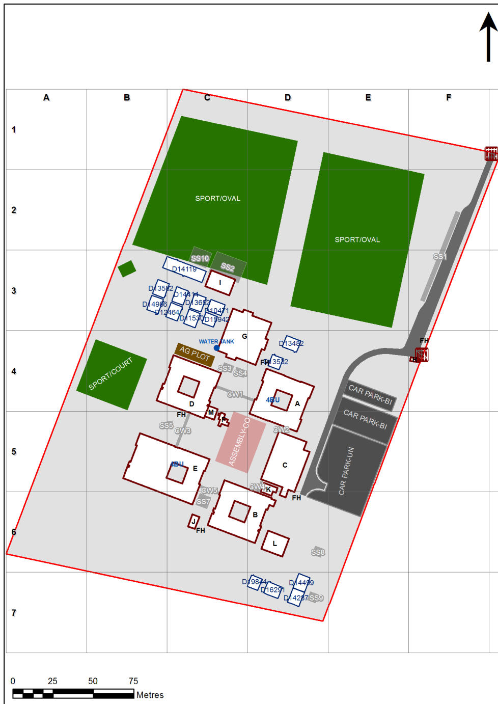
8401 - Lurnea High School Site Plan (11183)
