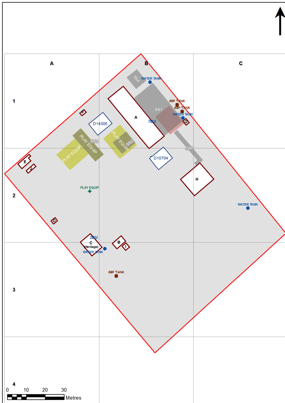
2431 - Luddenham Public School Site Plan (12773)
