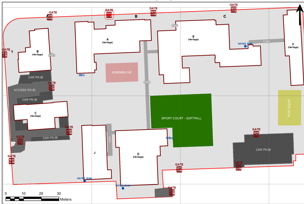
7423 - Leichhardt Public School Site Plan (12761)
