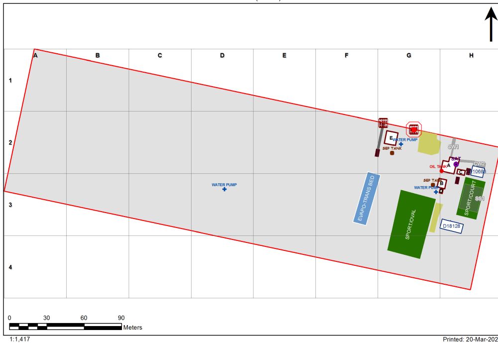
2273 - Kellys Plains Public School Site Plan (12568)
