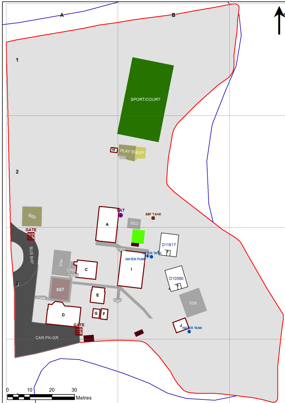
2260 - Karangi Public School Site Plan (12961)
