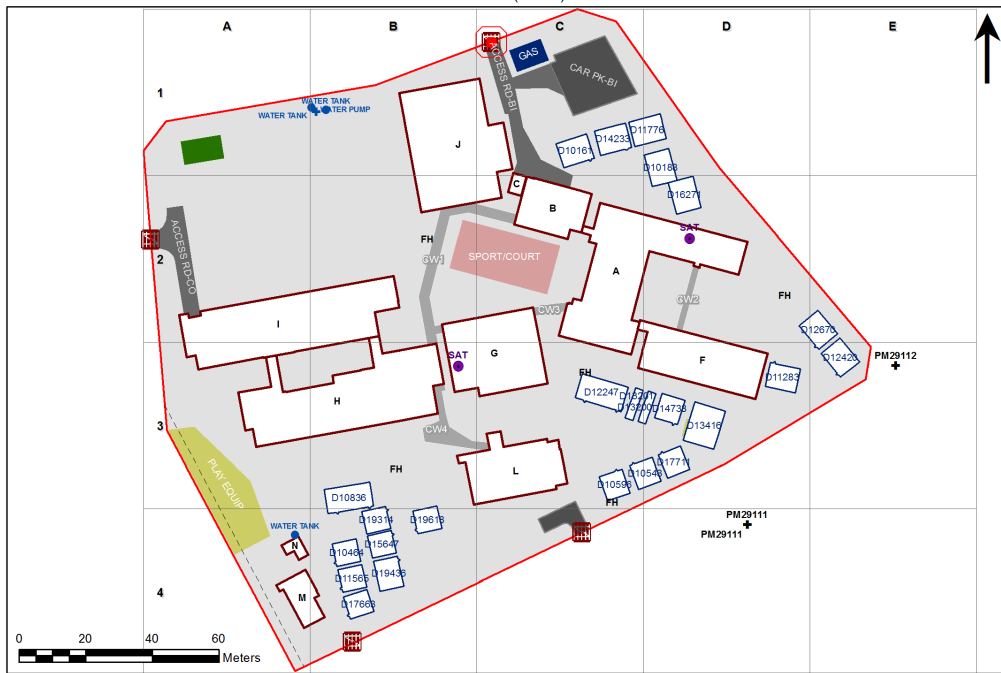
2237 - Jindabyne Central School Site Plan (10444)
