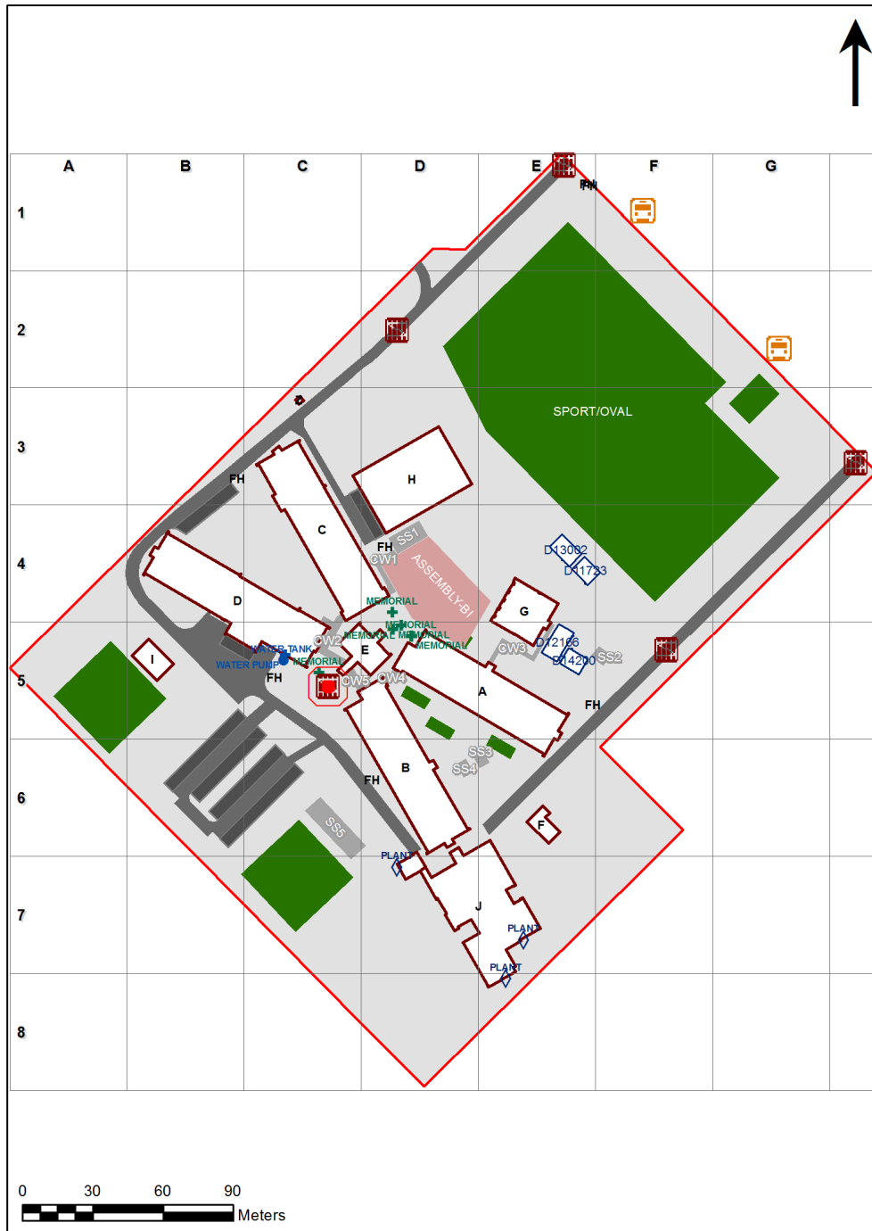
8262 - Ingleburn High School Site Plan (10758)
