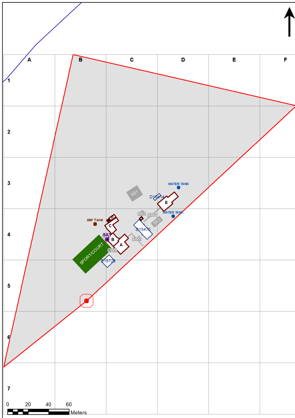
2190 - Huntingdon Public School Site Plan (11435)
