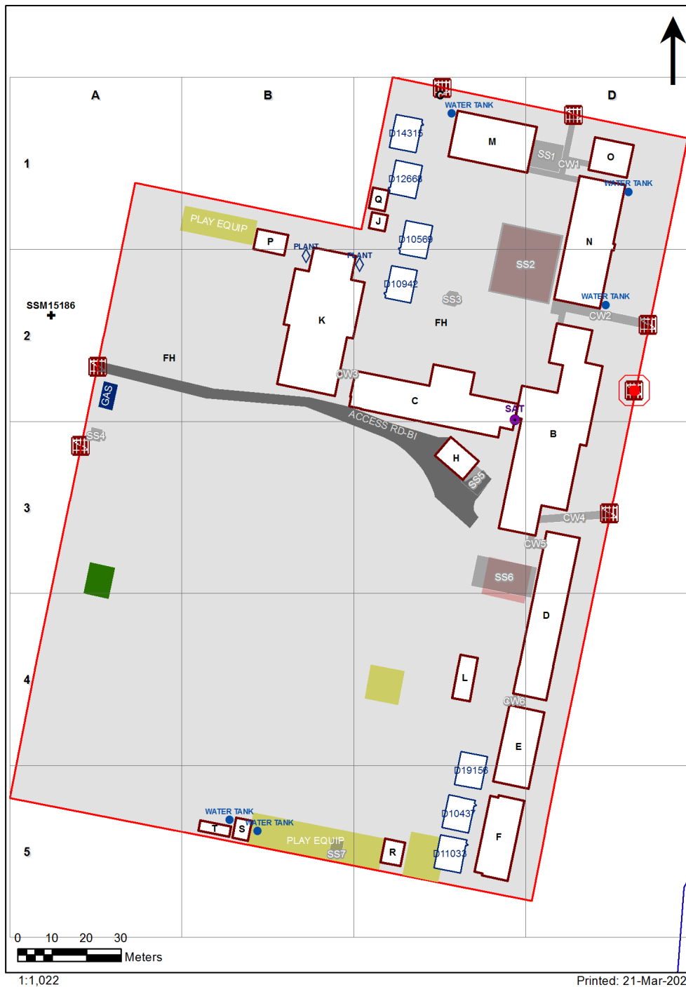
4018 - Gunnedah South Public School Site Plan (12705)
