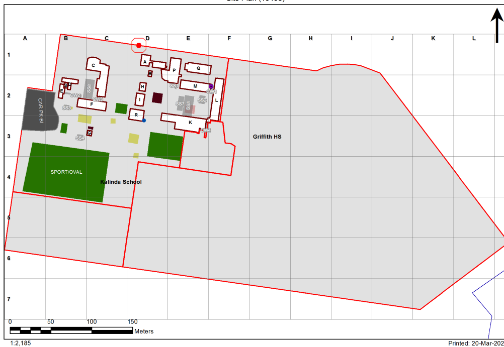
2087 - Griffith Public School Site Plan (10406)
