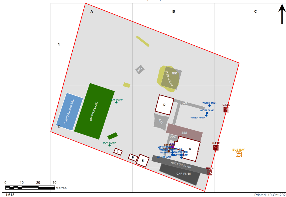
2020 - Glen William Public School Site Plan (11769)
