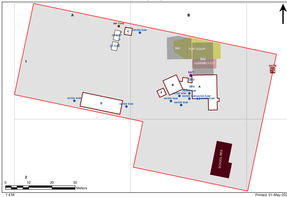
3903 - Glen Alice Public School Site Plan (12732)
