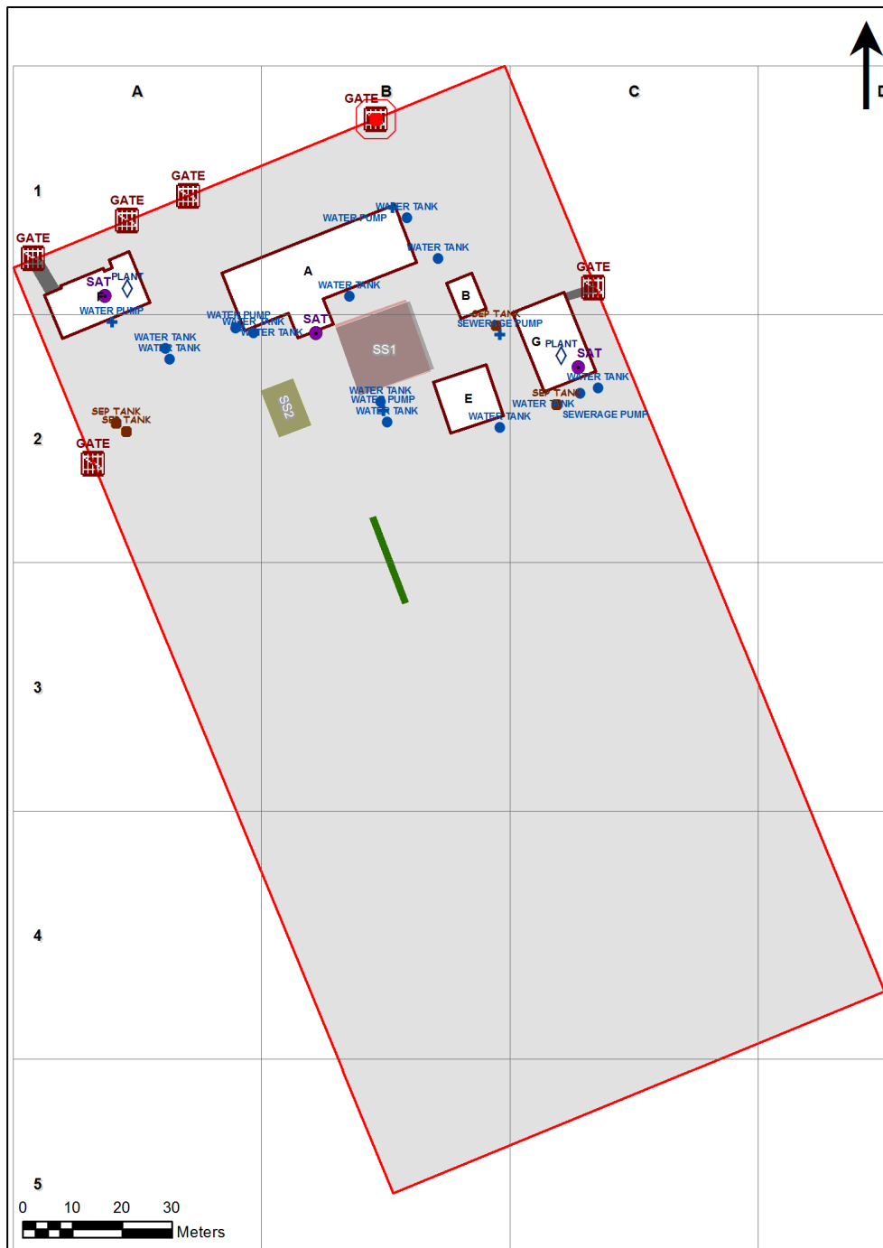
1956 - Garah Public School Site Plan (10592)
