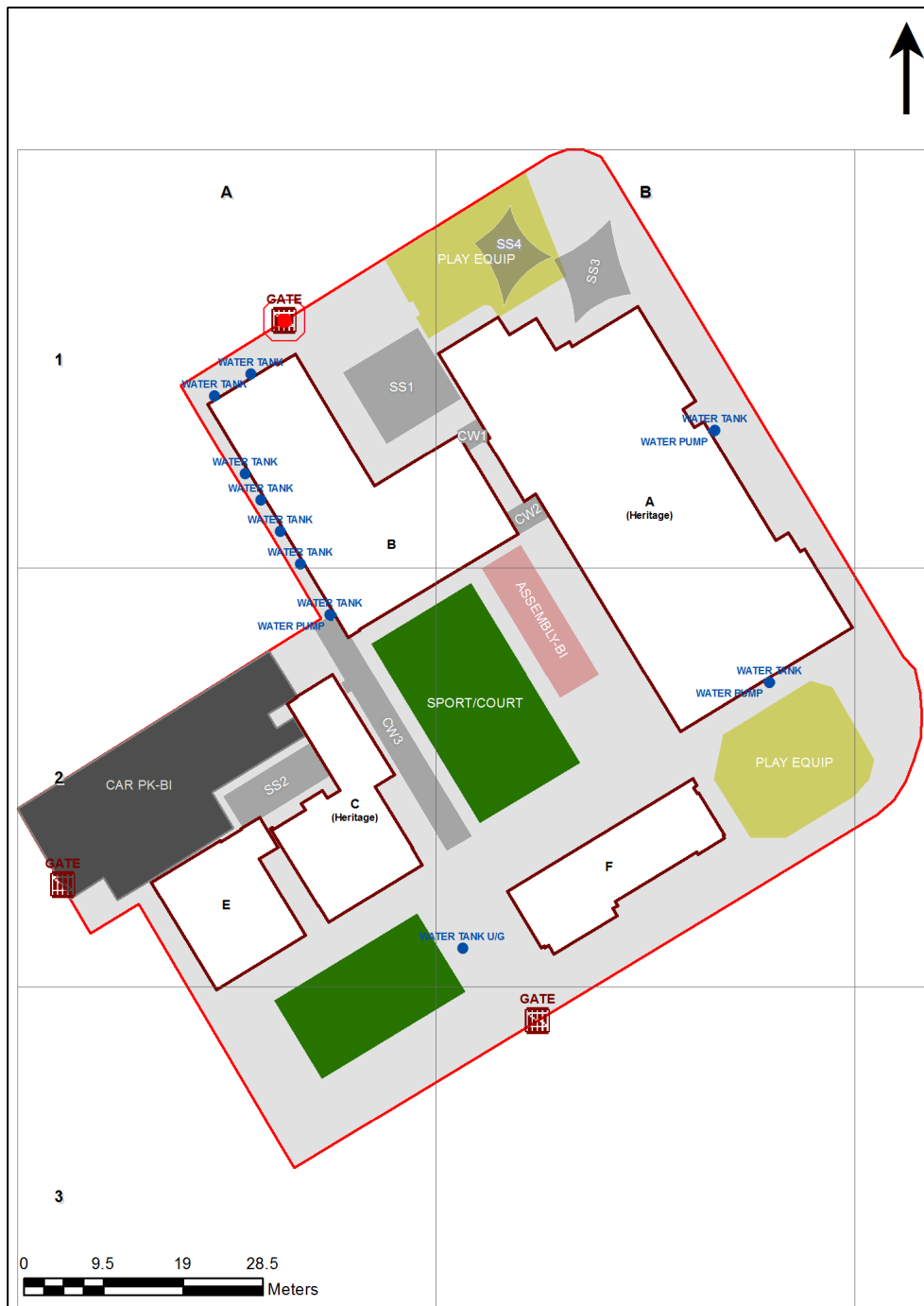
1932 - Forest Lodge Public School Site Plan (11877)
