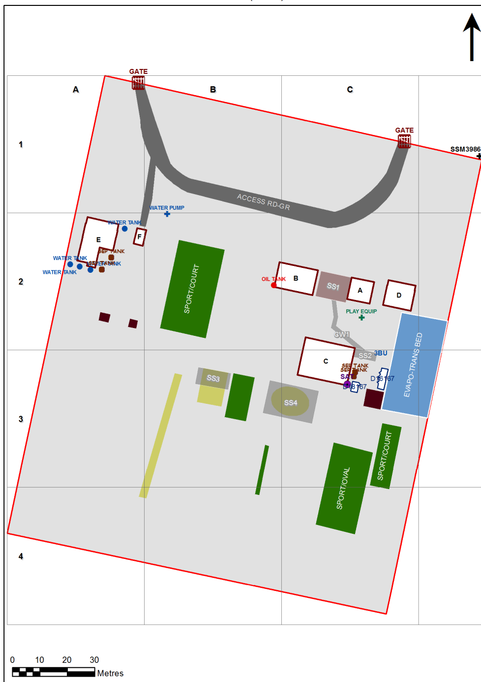
1802 - Duri Public School Site Plan (11931)
