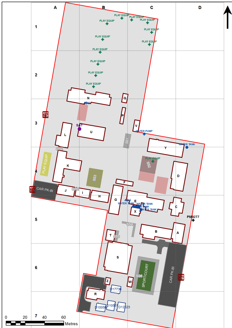
1811 - Dubbo South Public School Site Plan (13316)
