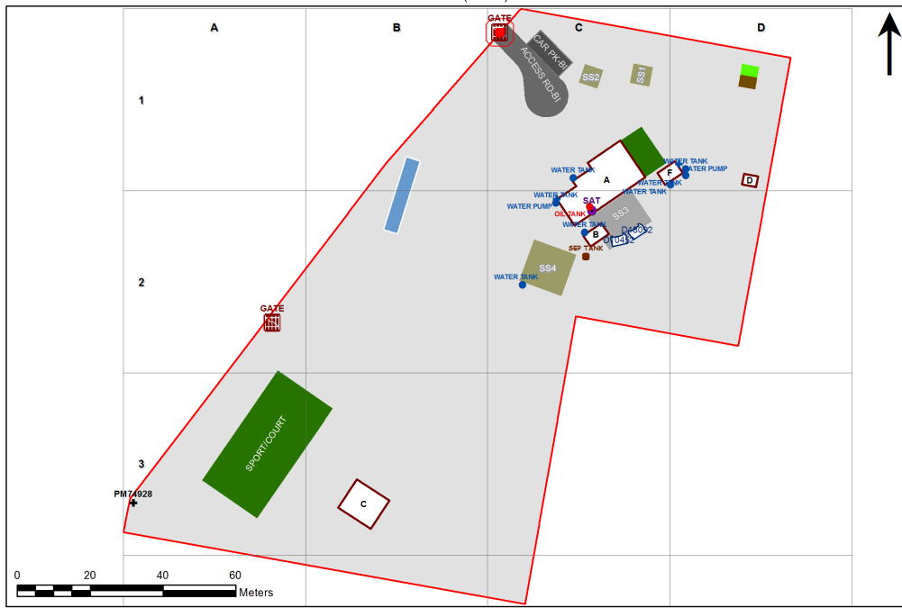
1822 - Congewai Public School Site Plan (11954)
