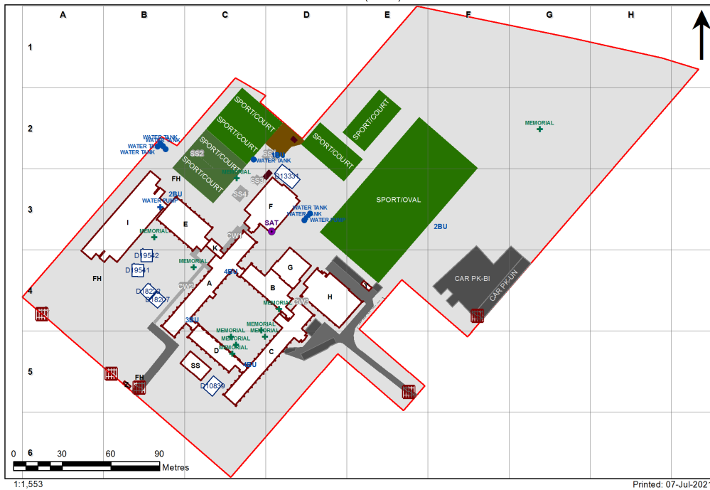
8208 - Cheltenham Girls High School Site Plan (10229)
