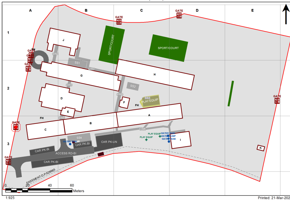
4607 - Centaur Public School Site Plan (13551)
