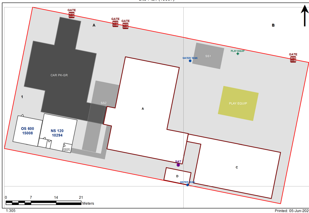
5749 - Budawang School Site Plan (13607)
