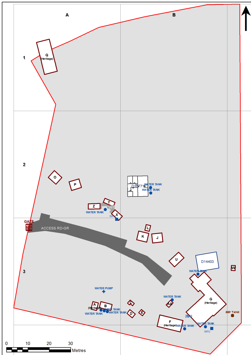
5694 - Brewongle Environmental Education Centre Site Plan (10114)
