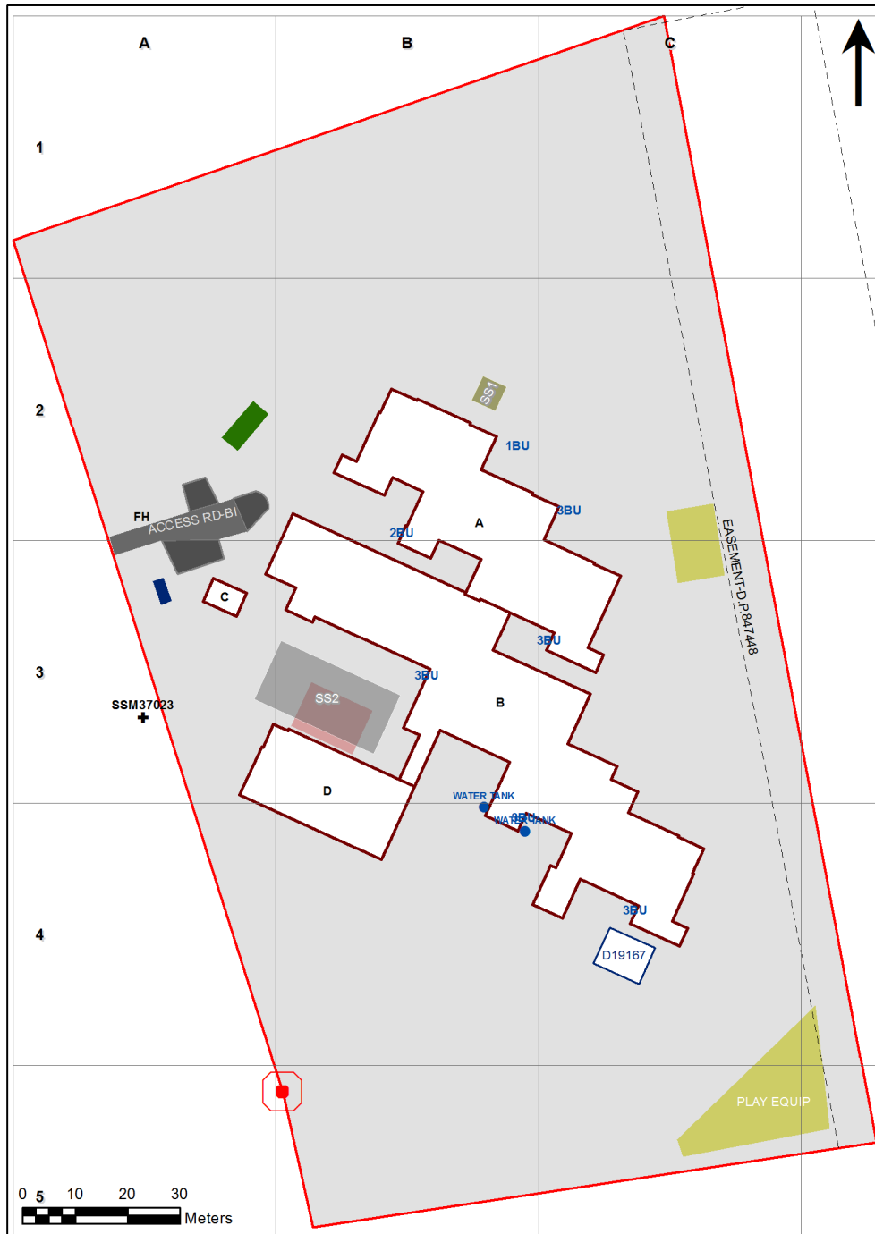
4507 - Bonnet Bay Public School Site Plan (10906)
