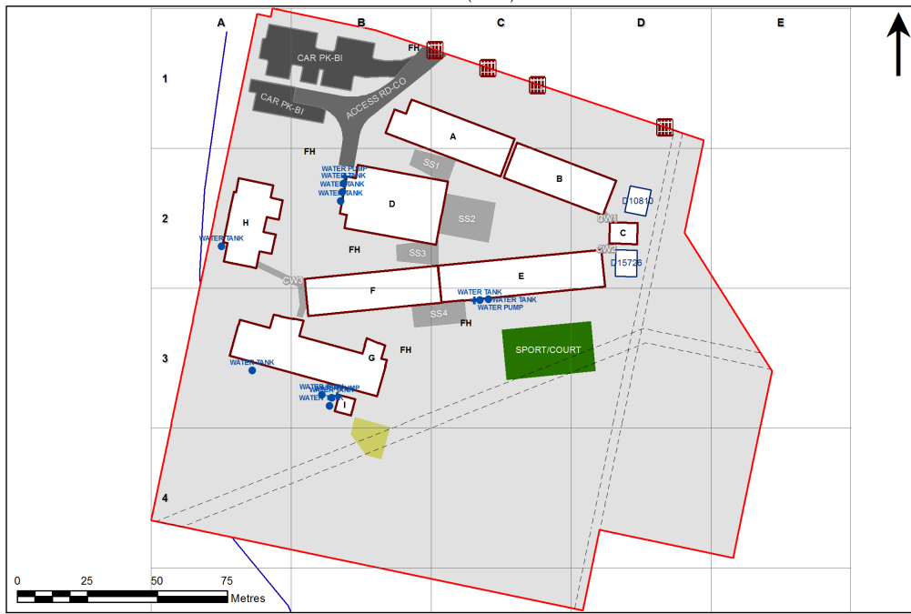
4623 - Blue Haven Public School Site Plan (13303)
