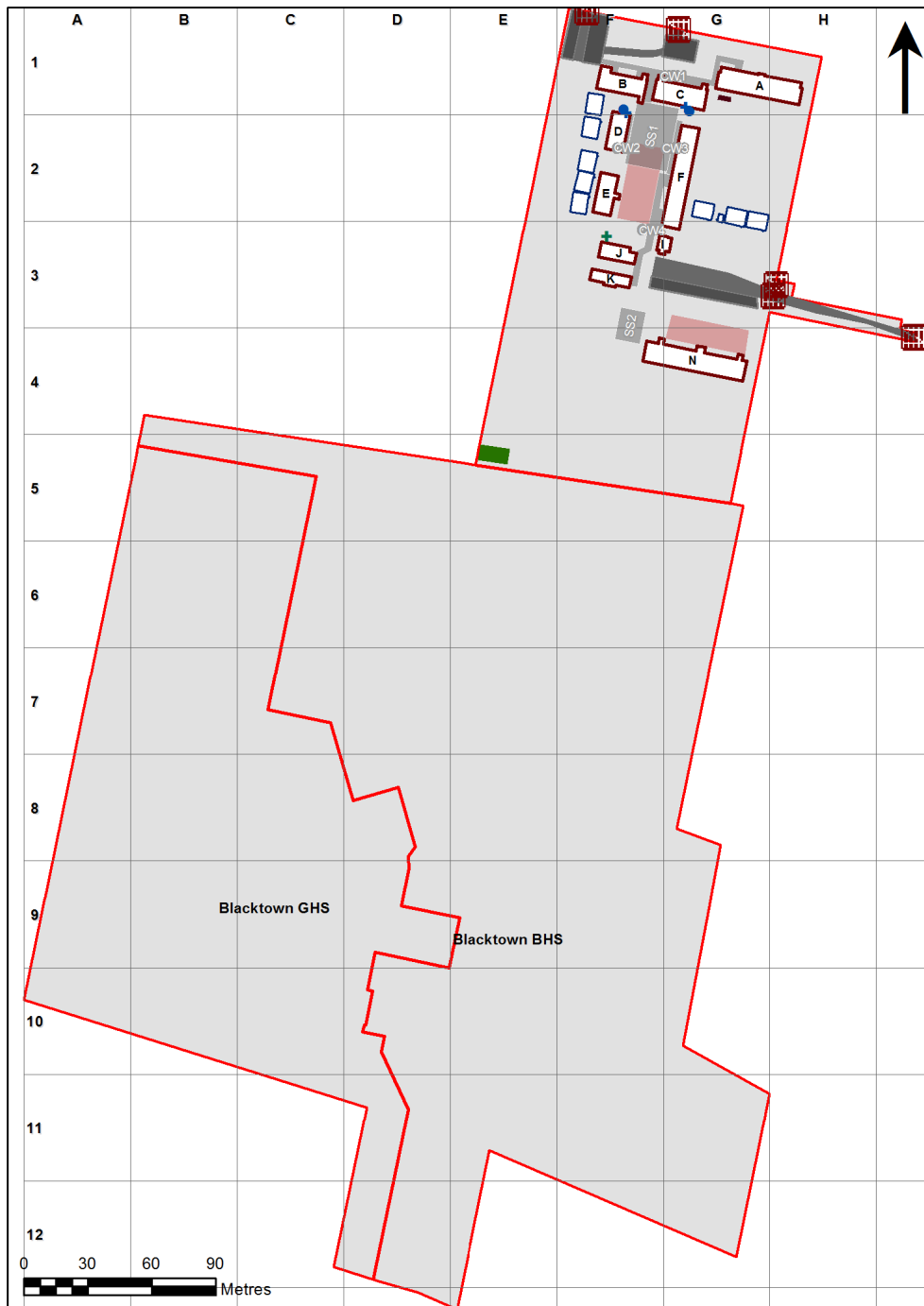
4061 - Blacktown North Public School Site Plan (10885)
