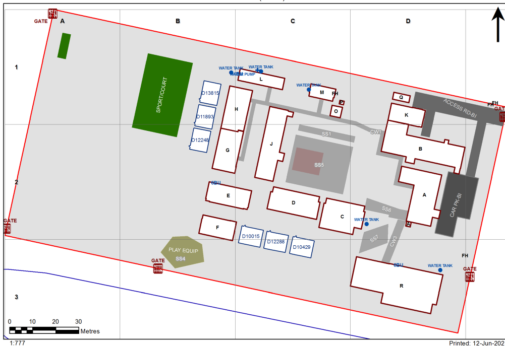
4057 - Birrong Public School Site Plan (10883)
