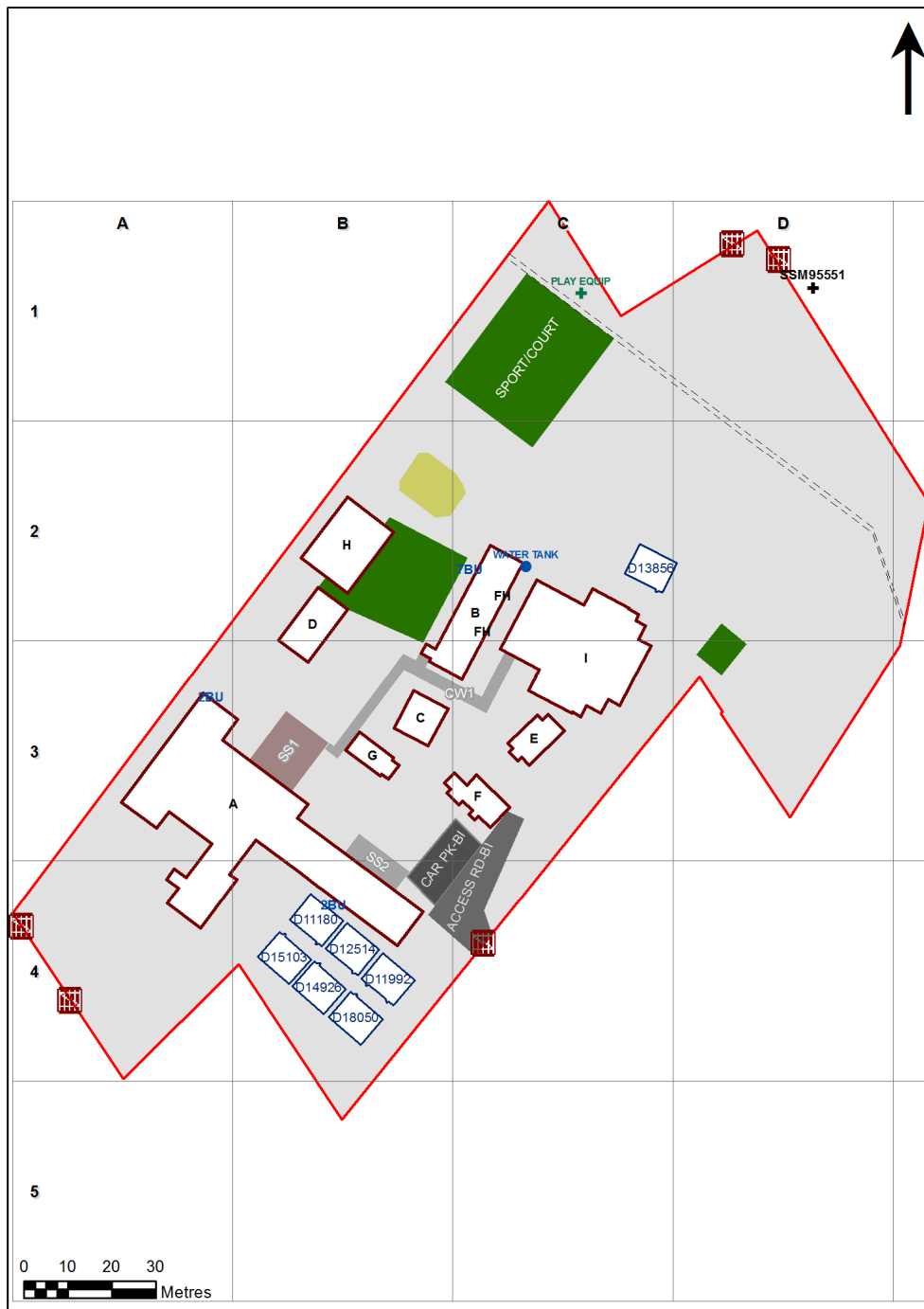
2308 - Bexley North Public School Site Plan (10219)
