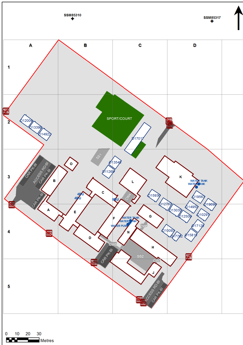
4377 - Baulkham Hills North Public School Site Plan (10198)
