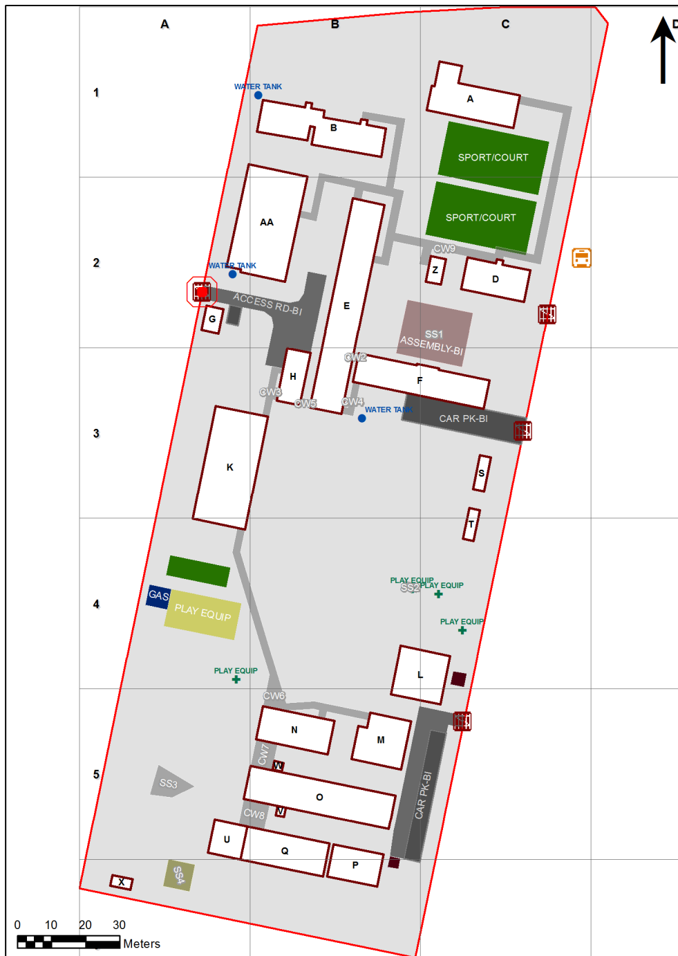
1148 - Bass Hill Public School Site Plan (13195)
