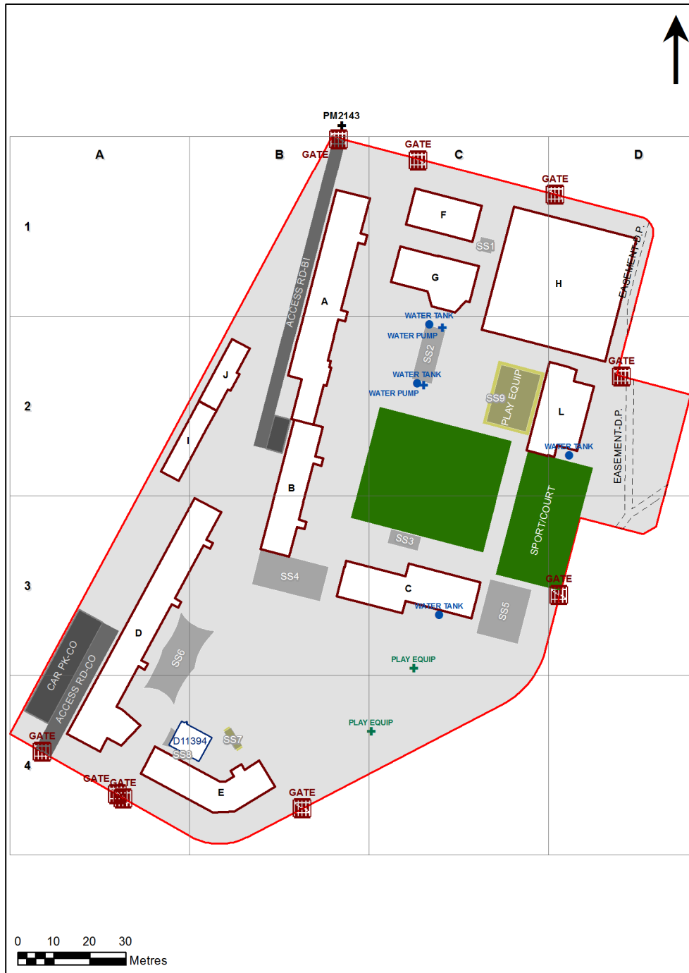
4200 - Allambie Heights Public School Site Plan (10588)
